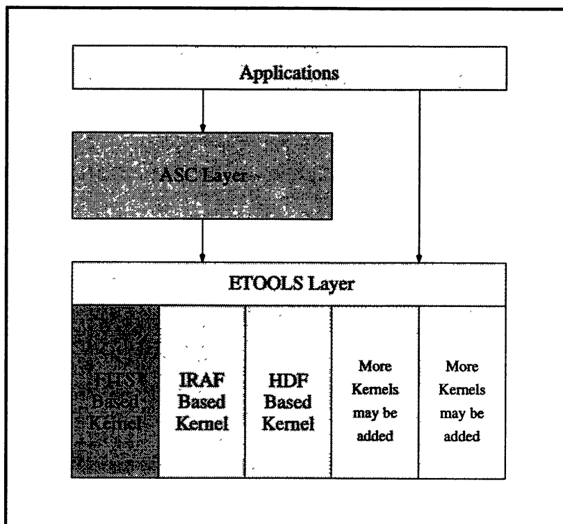
Figure 1. Layered Design of the ASC Data Model.
