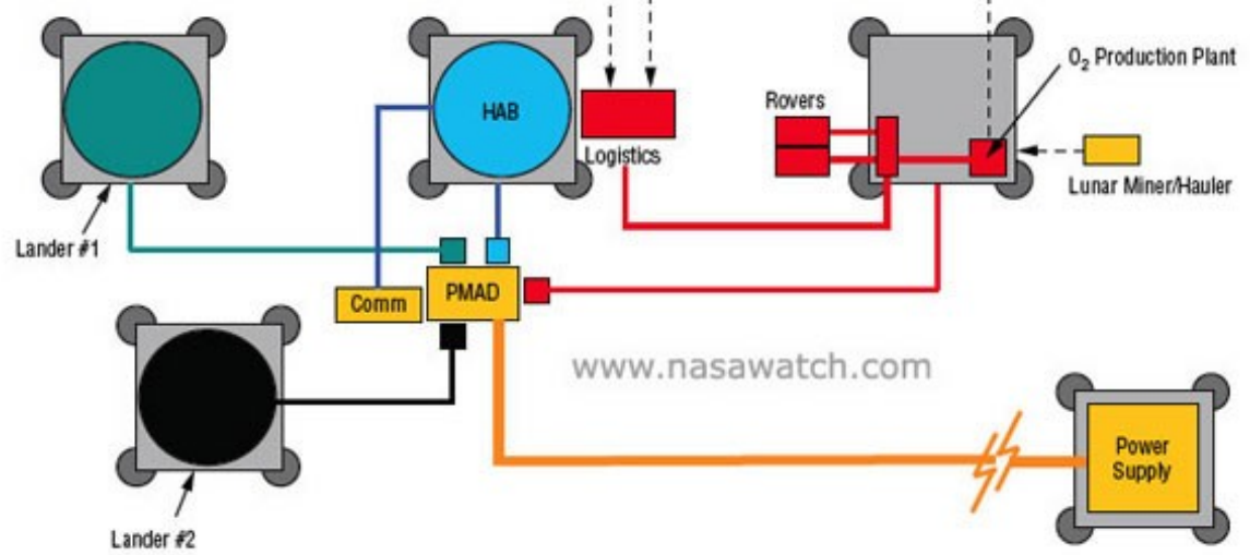
Figure 4-64. Core Outpost Schematic
